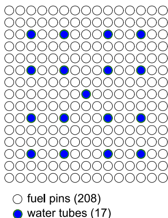
Figure 2.2. 15x15 UOX FA (with 17 water tubes)
