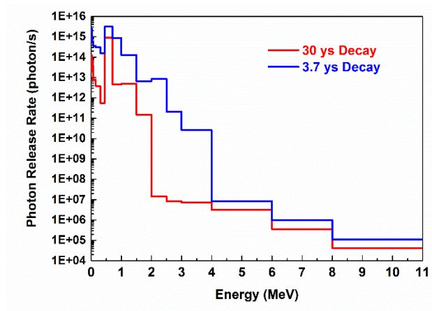
Figure A.3. UOX FA: \gamma source after 30 years and 3.7 years of decay vs. energy
