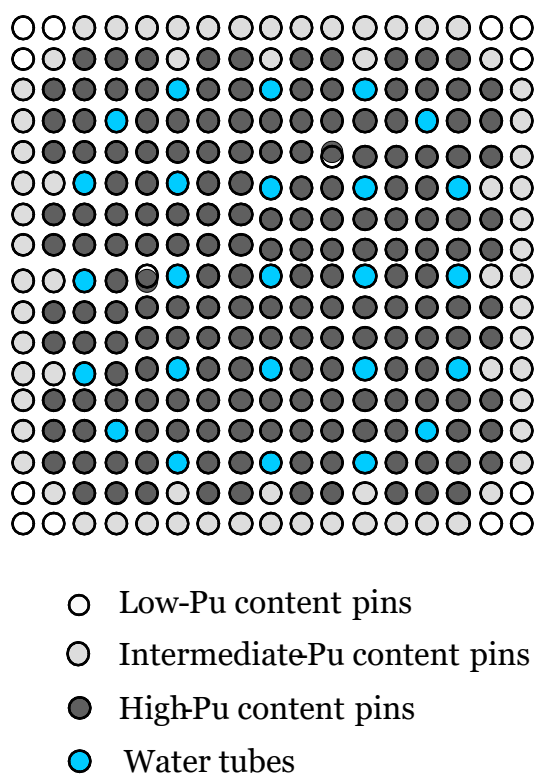
Figure 2.3. 17x17 MOX FA
