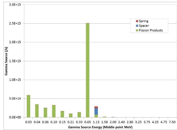
Figure 7.8. B03 FA: Calculated gamma source spectra featuring ray-line from ^{60}\text{Co} decay
