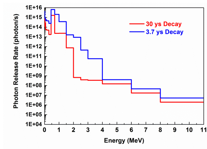
Figure A.7. UOX FA: \gamma source after 30 years and 3.7 years of decay vs. energy
