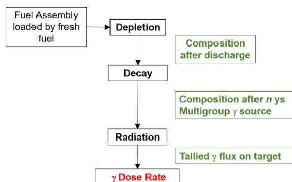
Figure A.1. Flow chart of the calculation procedure for \gamma dose rate evaluation
