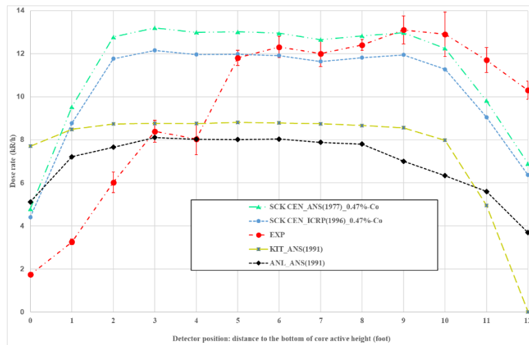
Figure 7.39. Calculated versus experimental dose rates inside the axial holder tube 30.48 cm away from the surface of the B03 assembly
